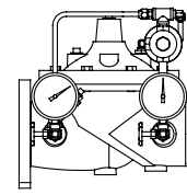
ZW209FPX Class 150 Flanged Max 250 psi Inlet
