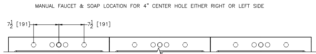
TOP VIEW
