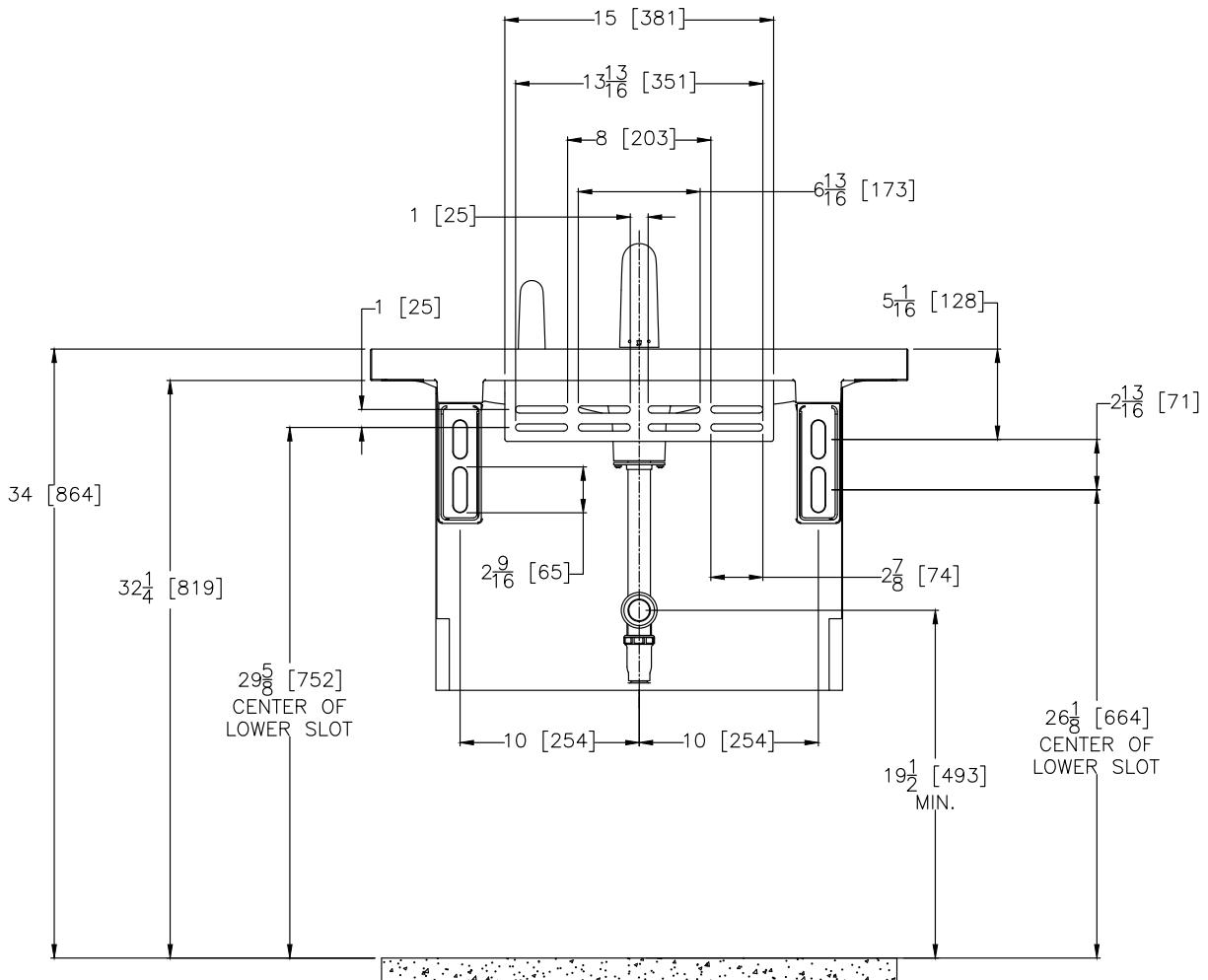
BRACKET VIEW
