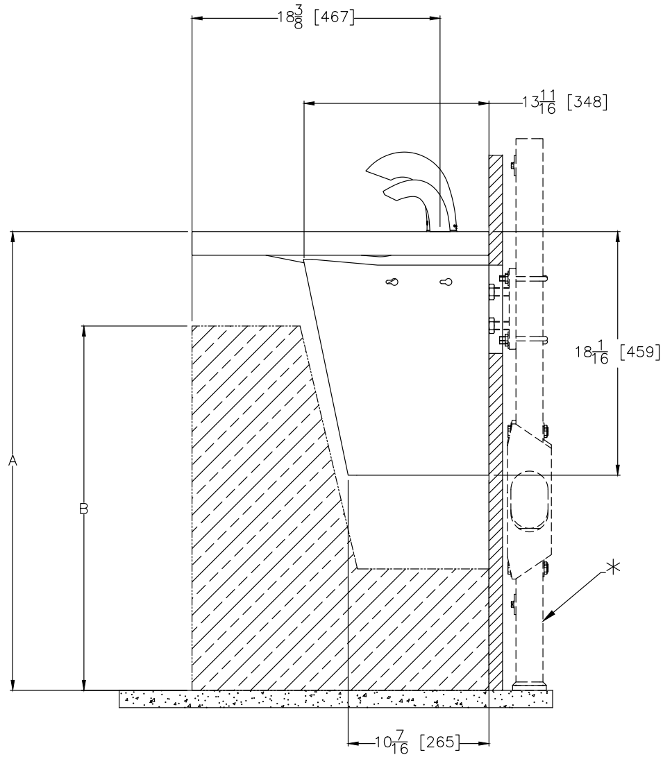
SIDE VIEW
