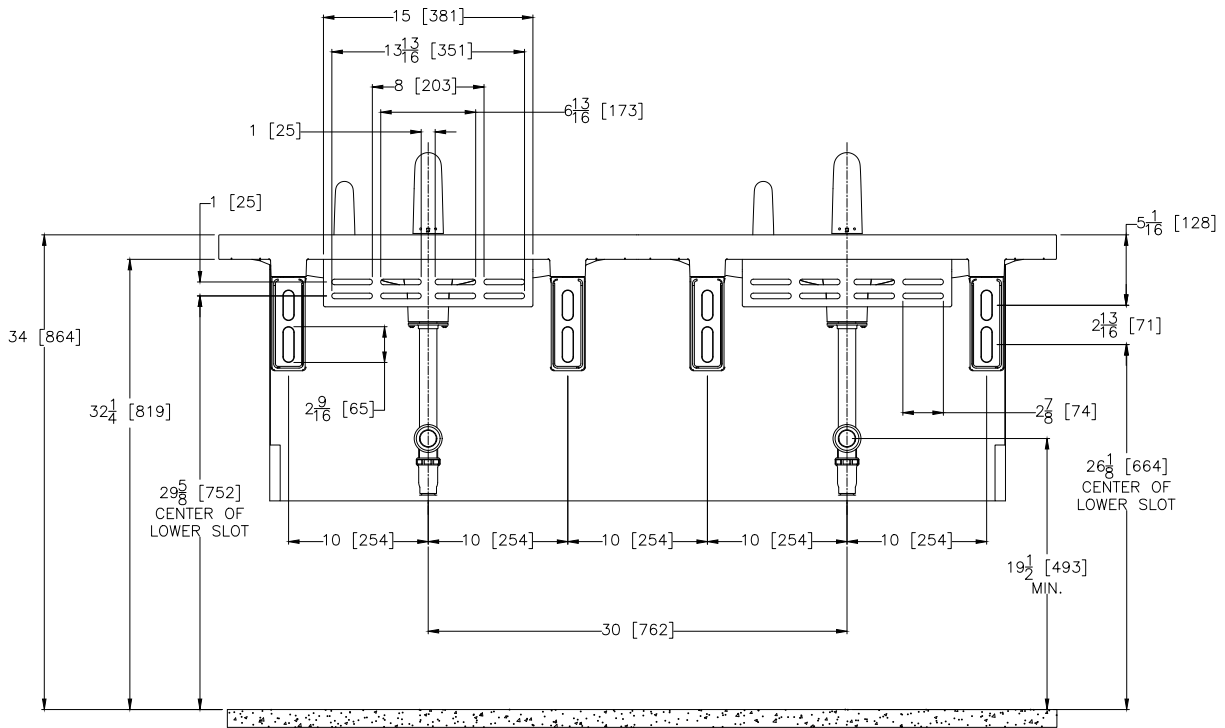
BRACKET VIEW
