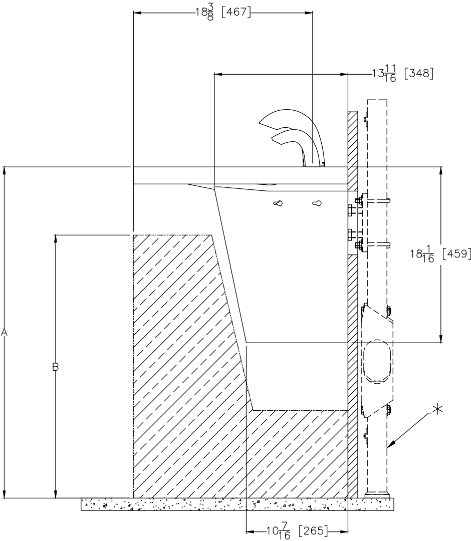
SIDE VIEW
