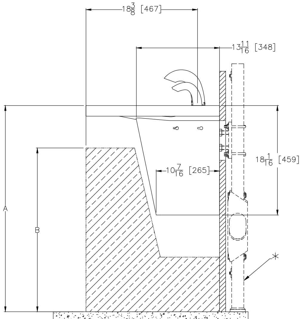
SIDE VIEW
