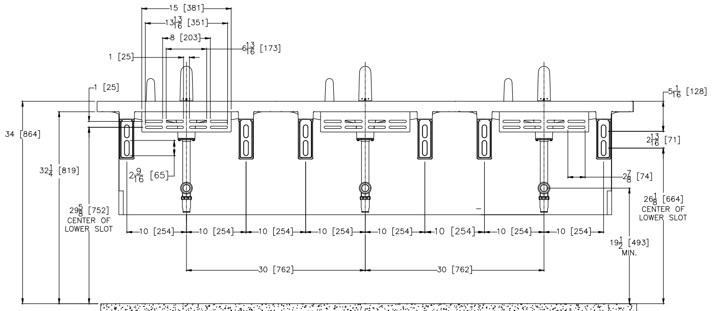
BRACKET VIEW
