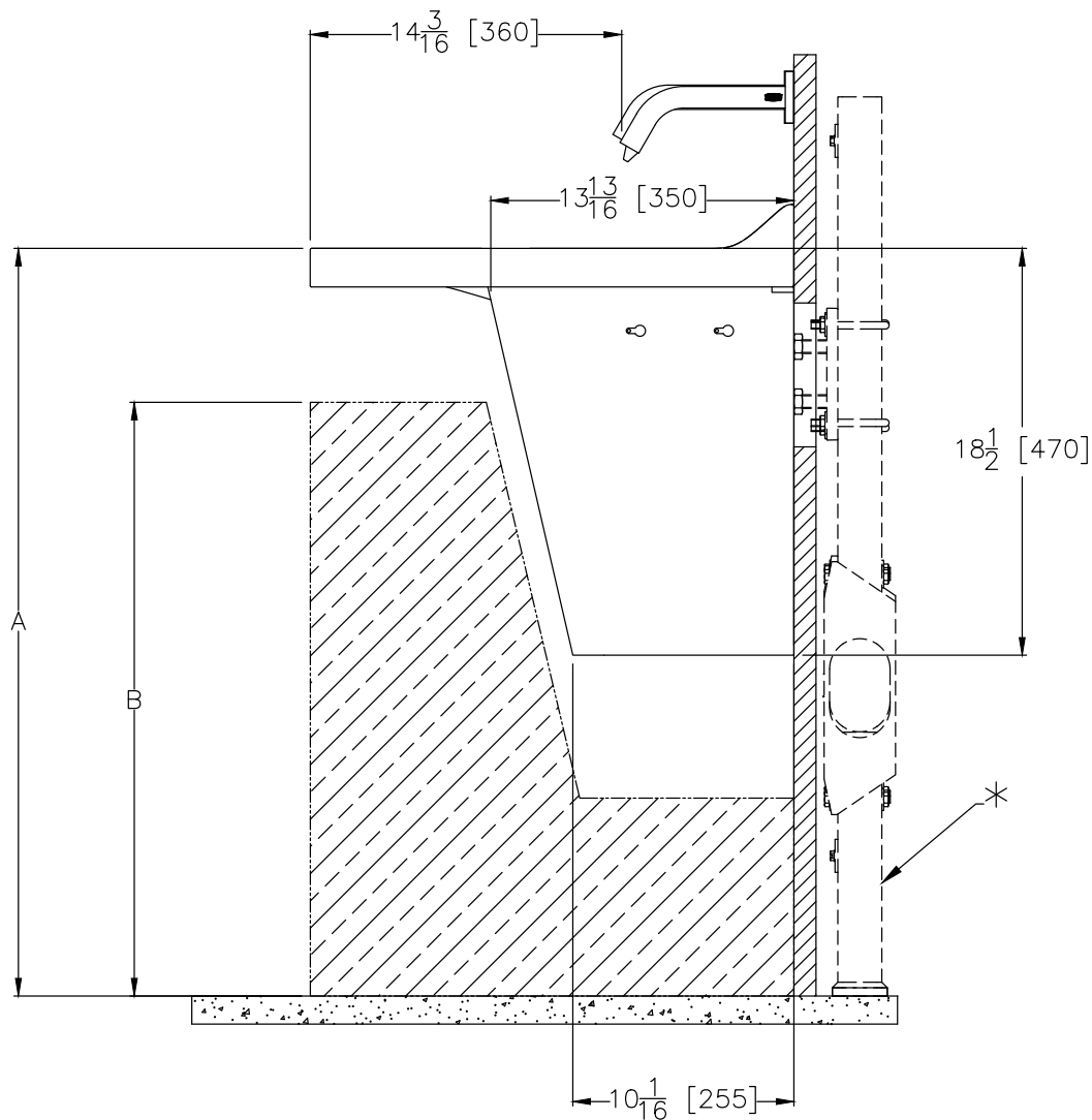
SIDE VIEW
