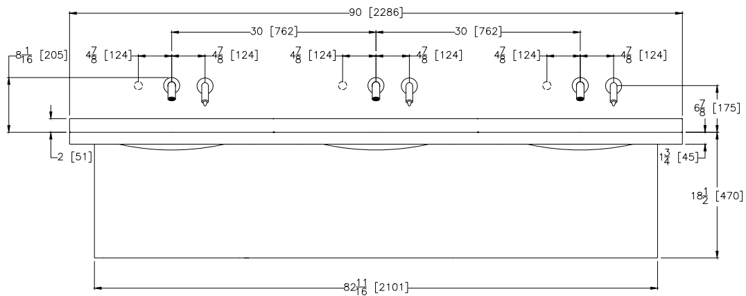
FRONT VIEW
