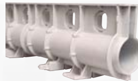
Z888-4 Slotted Drainage System for 4" Pipe or Equivalent
