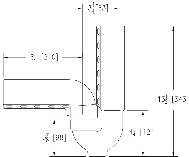
TRAP PROTECTOR
